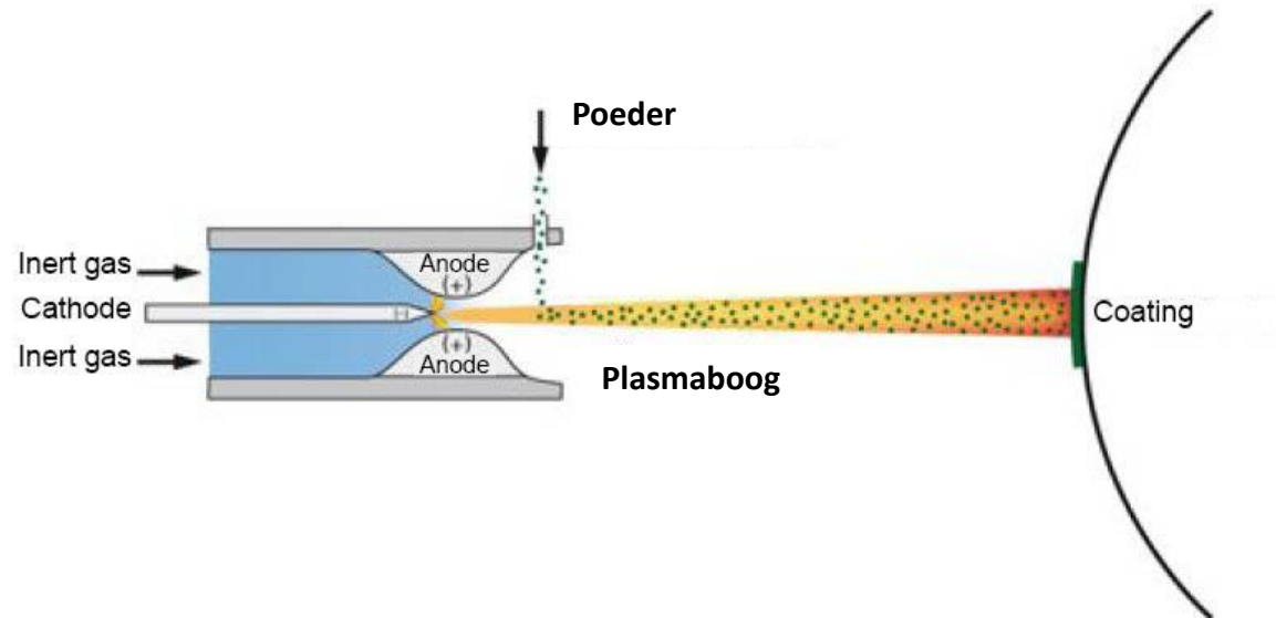
Plasmaspuiten (APS/VPS/APSS): Techniek
